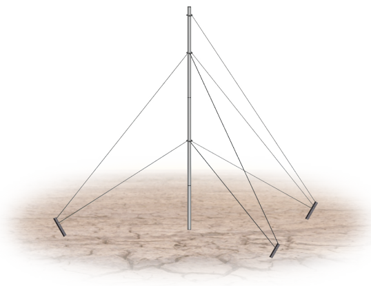
10m Premium Mast Setup
