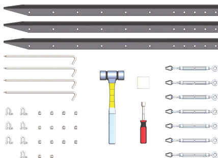
Guyed 10m Premium Mast - Tools
