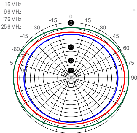
Relative Azimuth Pattern at EL -60° (9390 at 5m over ideal ground)
